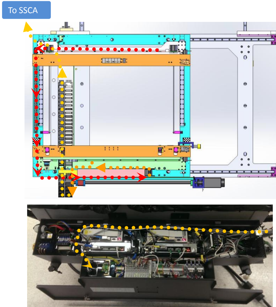
Figure 3 Right Stepper Motor Cable Routing
