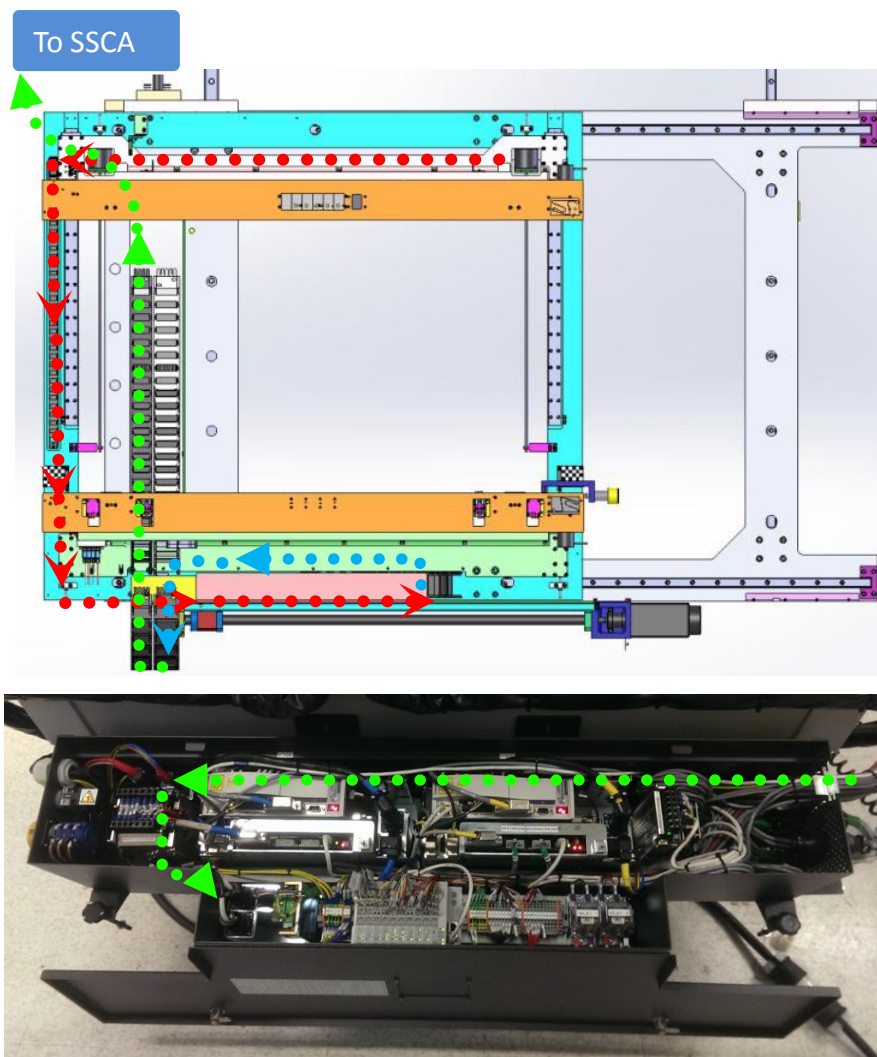
Figure 29 Stepper Motor Cable Routing
