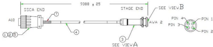
Figure 28 Cable Drawing
