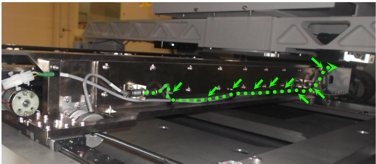
Figure 31 Stepper Motor Cable Routing
